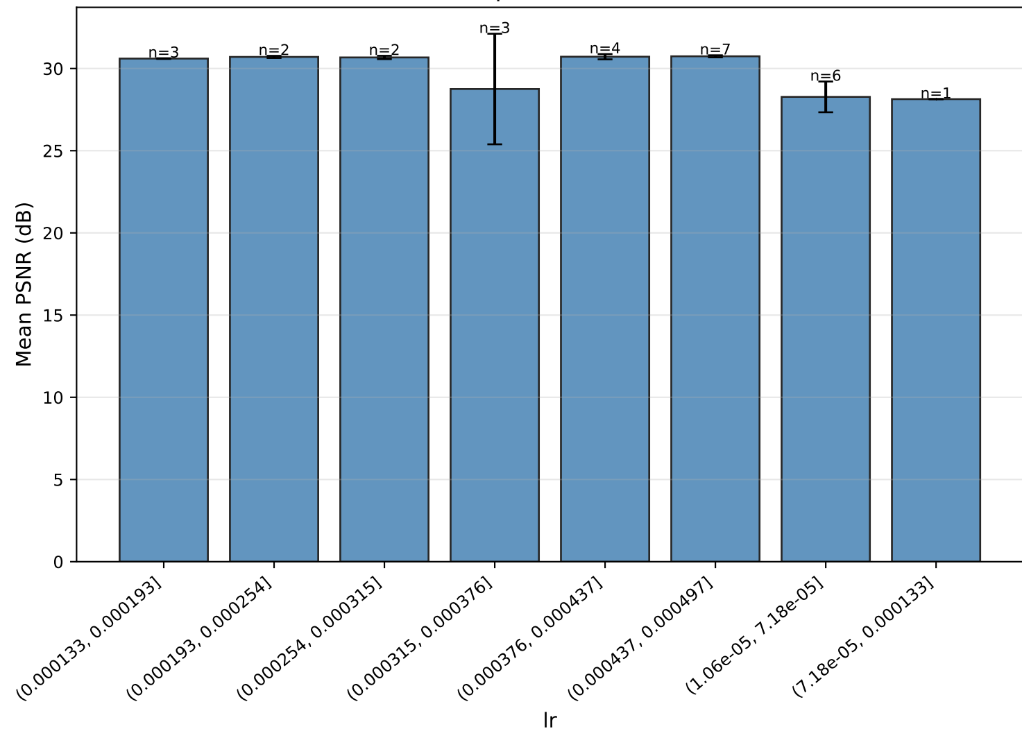
Mean PSNR per value of l_r — HAT
